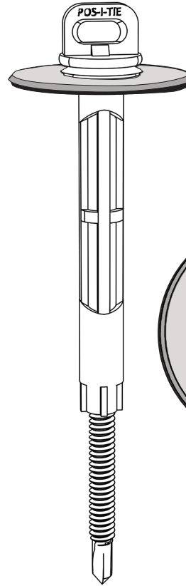
Apply Large Washer to factory assembled Pos-I-Tie® (Large washer should be flush against existing washer)*
