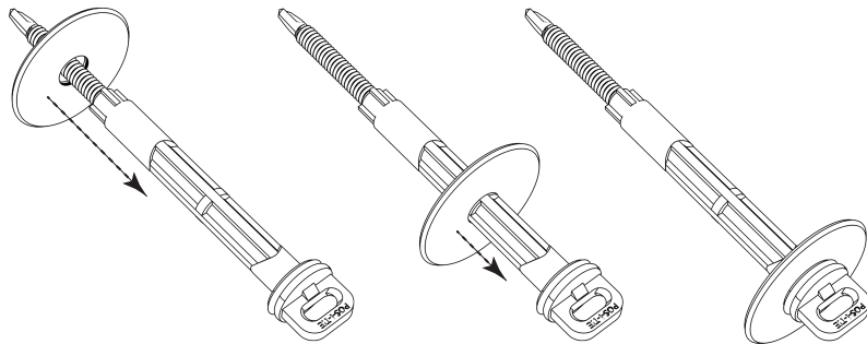
Apply Large Washer to factory assembled Pos-I-Tie® (Large washer should be flush against existing washer)*
